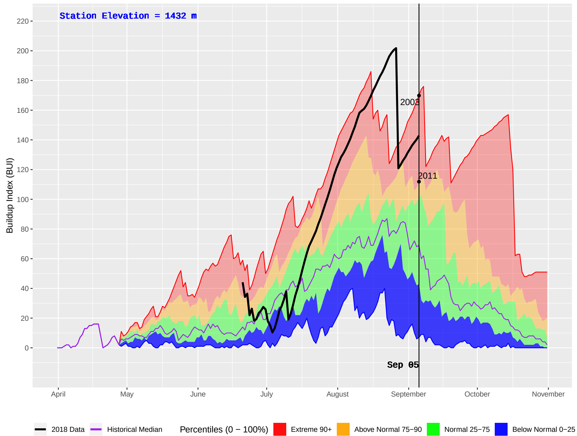
OCTOPUS CREEK (396) : Historical (2000–2016) and Current (2018) Daily Buildup Index (BUI)
